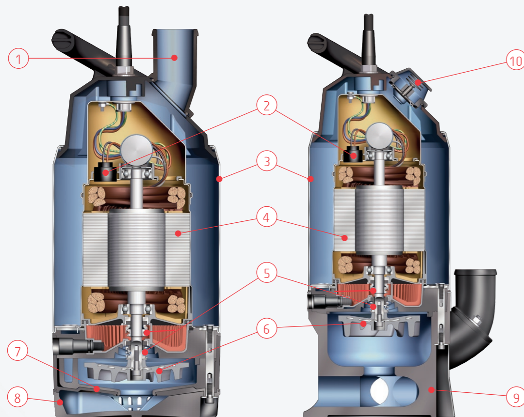
Drainage pump
